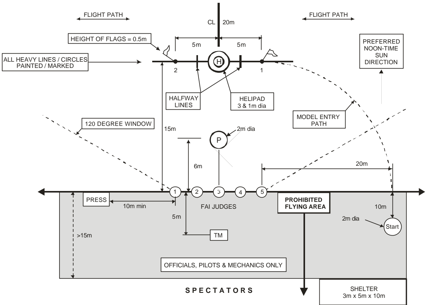
FIGURE 5.4.A - F3C CONTEST AREA LAYOUT
